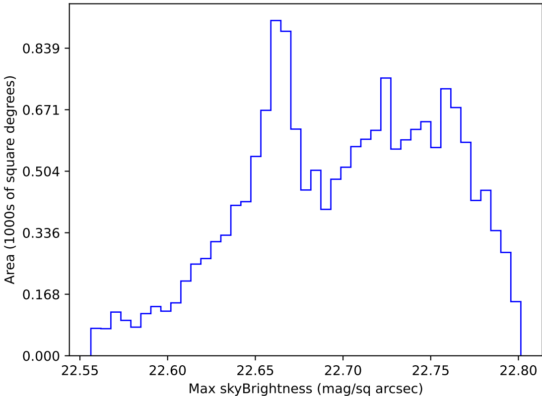
too_elab_r64_d3_gz_v3.4_10yrs WFD u band: Max skyBrightness
