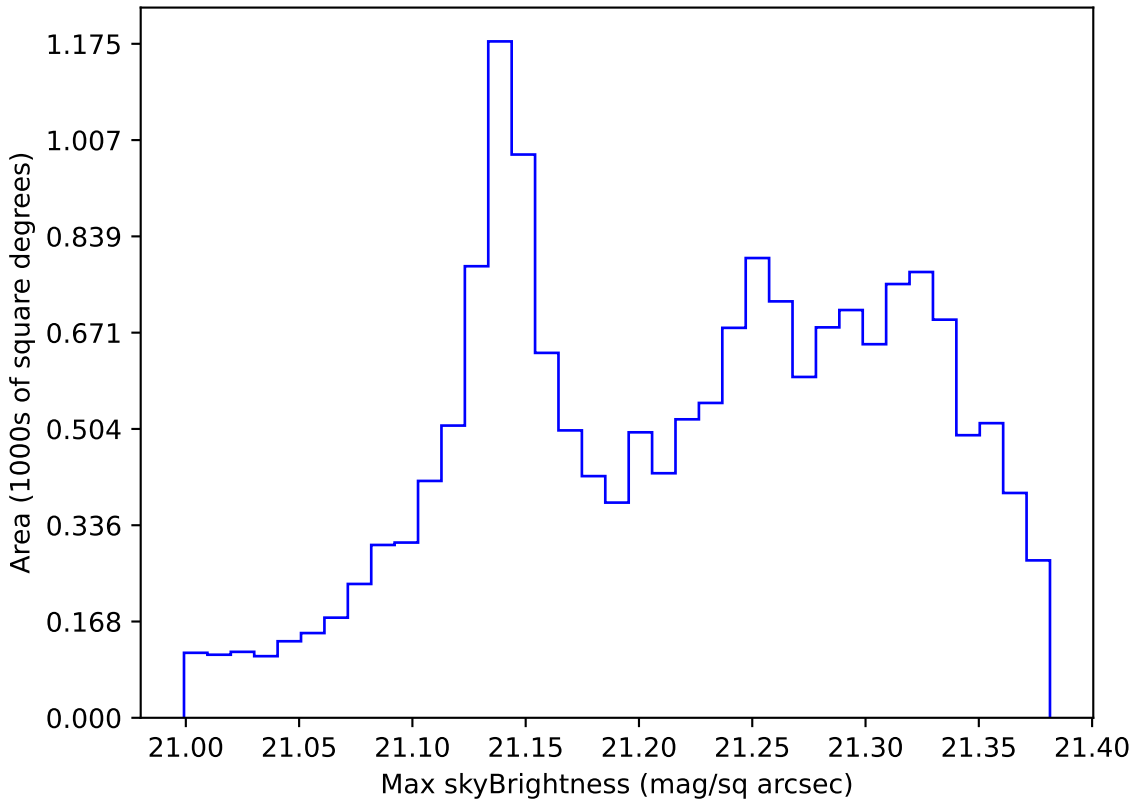
too_elab_r64_d3_gz_v3.4_10yrs WFD r band: Max skyBrightness
