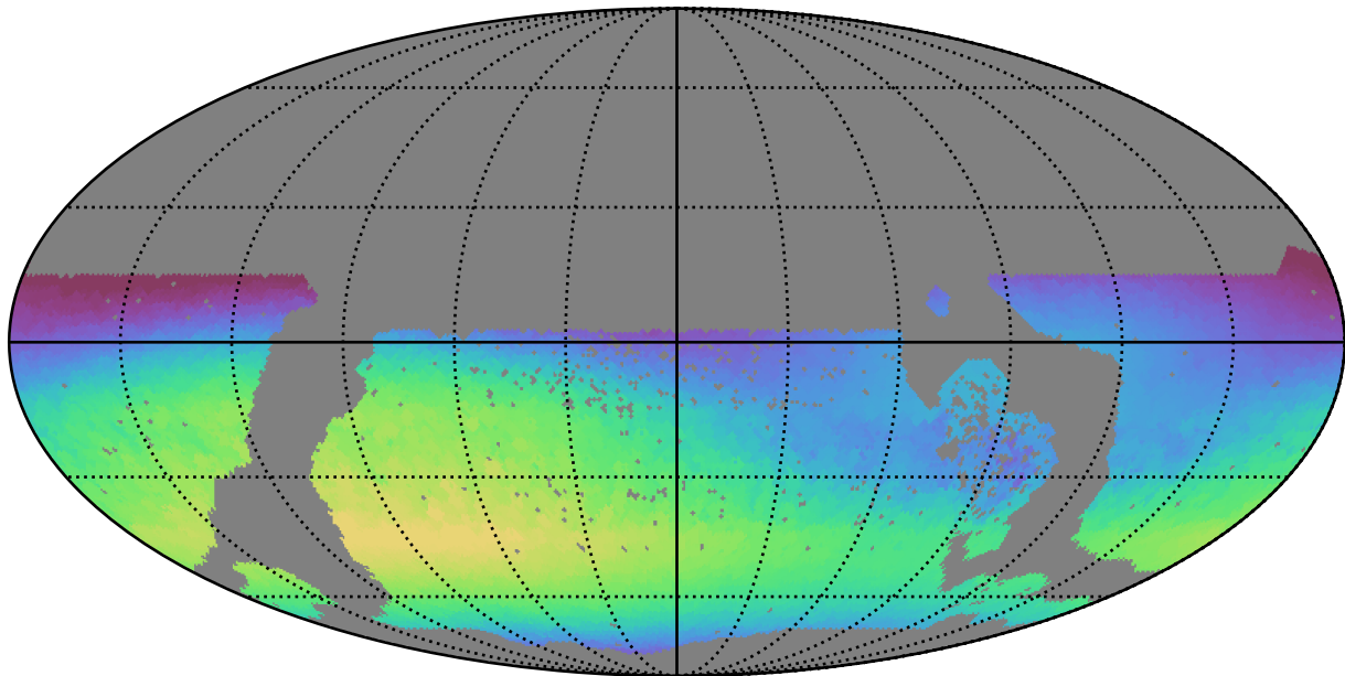
too_elab_r64_d3_gz_v3.4_10yrs WFD all bands: Max skyBrightness
