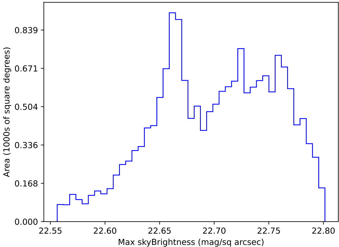
too_elab_r64_d3_gz_v3.4_10yrs WFD all bands: Max skyBrightness
