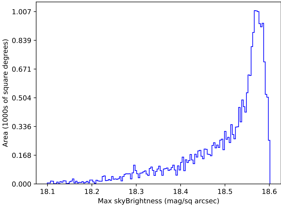
too_elab_r64_d3_gz_v3.4_10yrs All sky y band: Max skyBrightness
