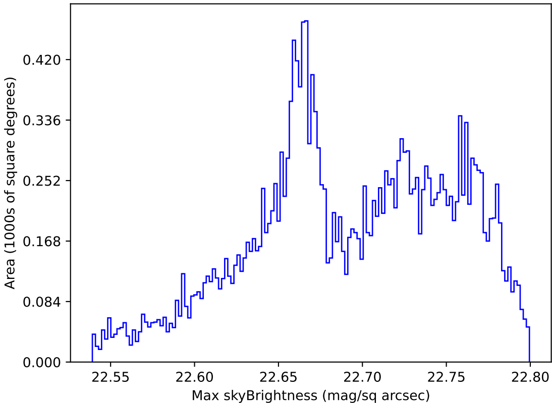
too_elab_r64_d3_gz_v3.4_10yrs All sky u band: Max skyBrightness
