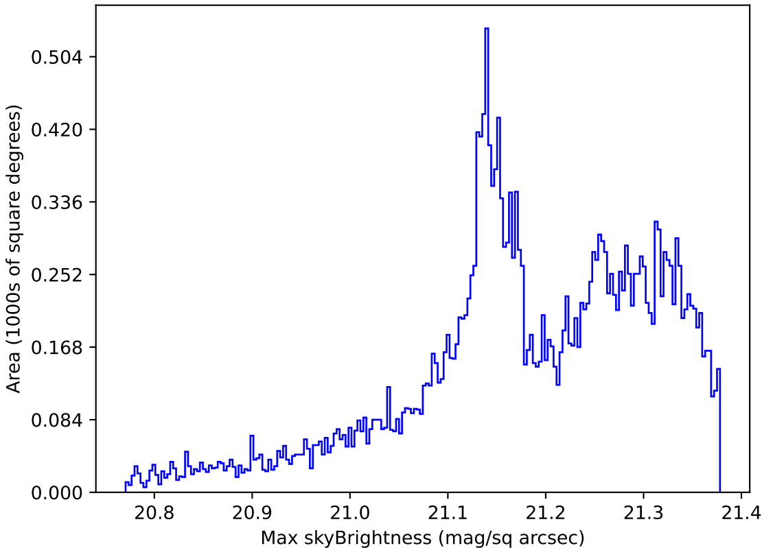
too_elab_r64_d3_gz_v3.4_10yrs All sky r band: Max skyBrightness
