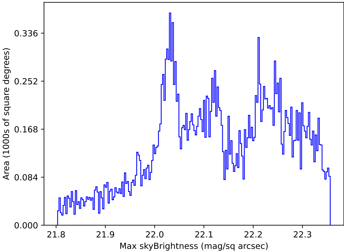
too_elab_r64_d3_gz_v3.4_10yrs All sky g band: Max skyBrightness
