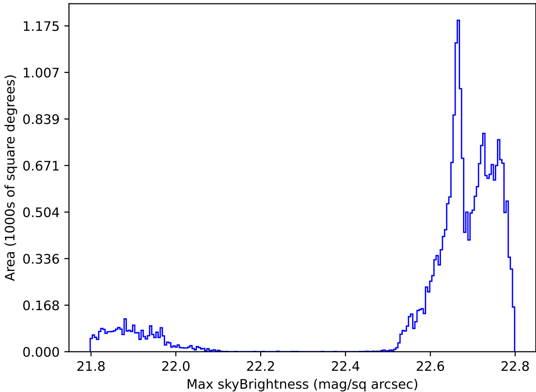
too_elab_r64_d3_gz_v3.4_10yrs All sky all bands: Max skyBrightness
