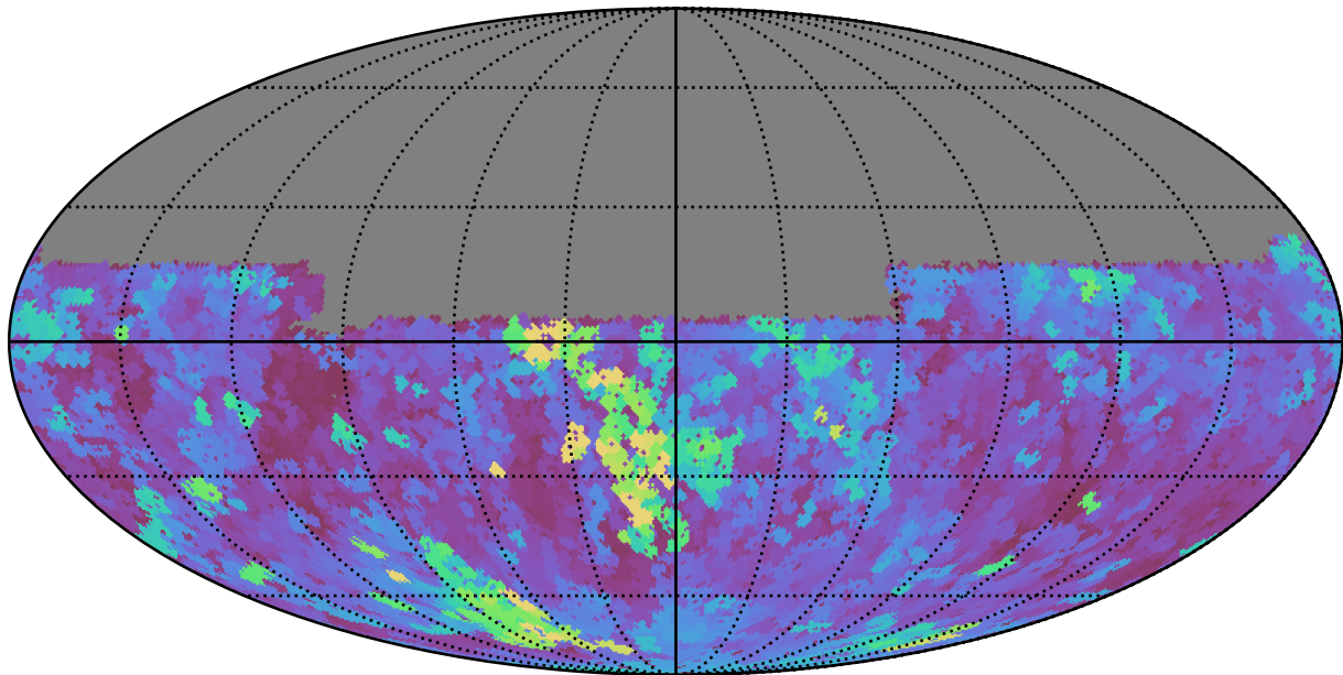
too_elab_r64_d3_gz_v3.4_10yrs Yr 1 y band: Max seeingGeom
