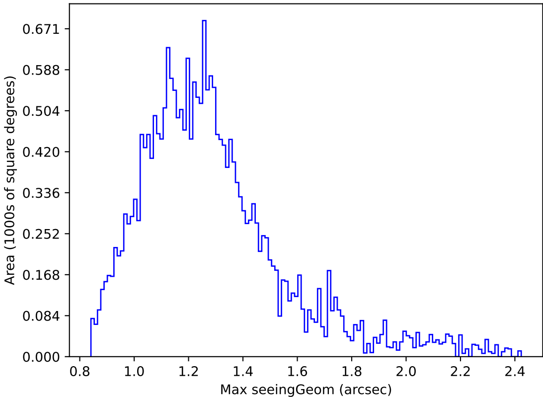
too_elab_r64_d3_gz_v3.4_10yrs Yr 1 y band: Max seeingGeom
