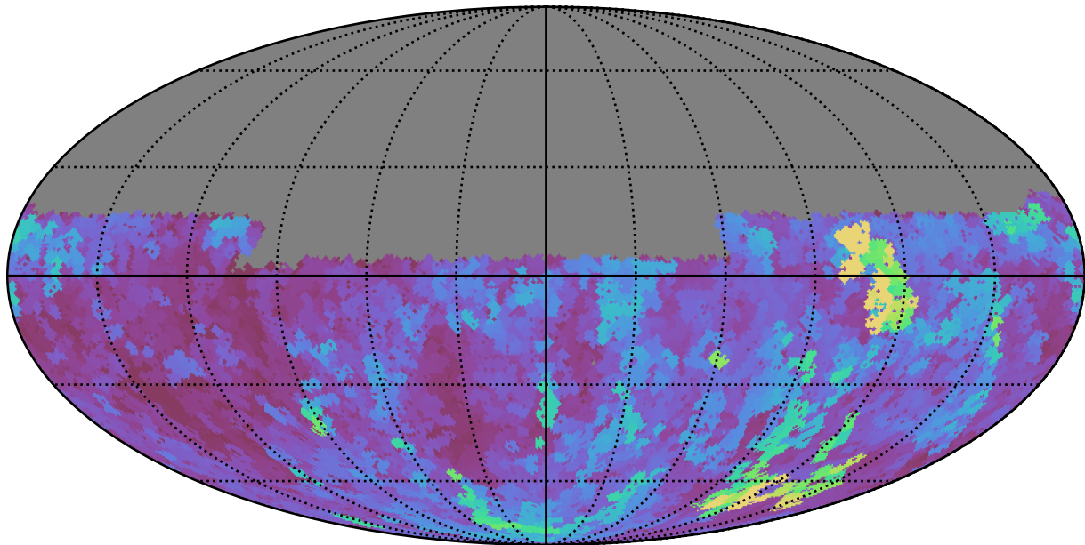
too_elab_r64_d3_gz_v3.4_10yrs Yr 1 u band: Max seeingGeom
