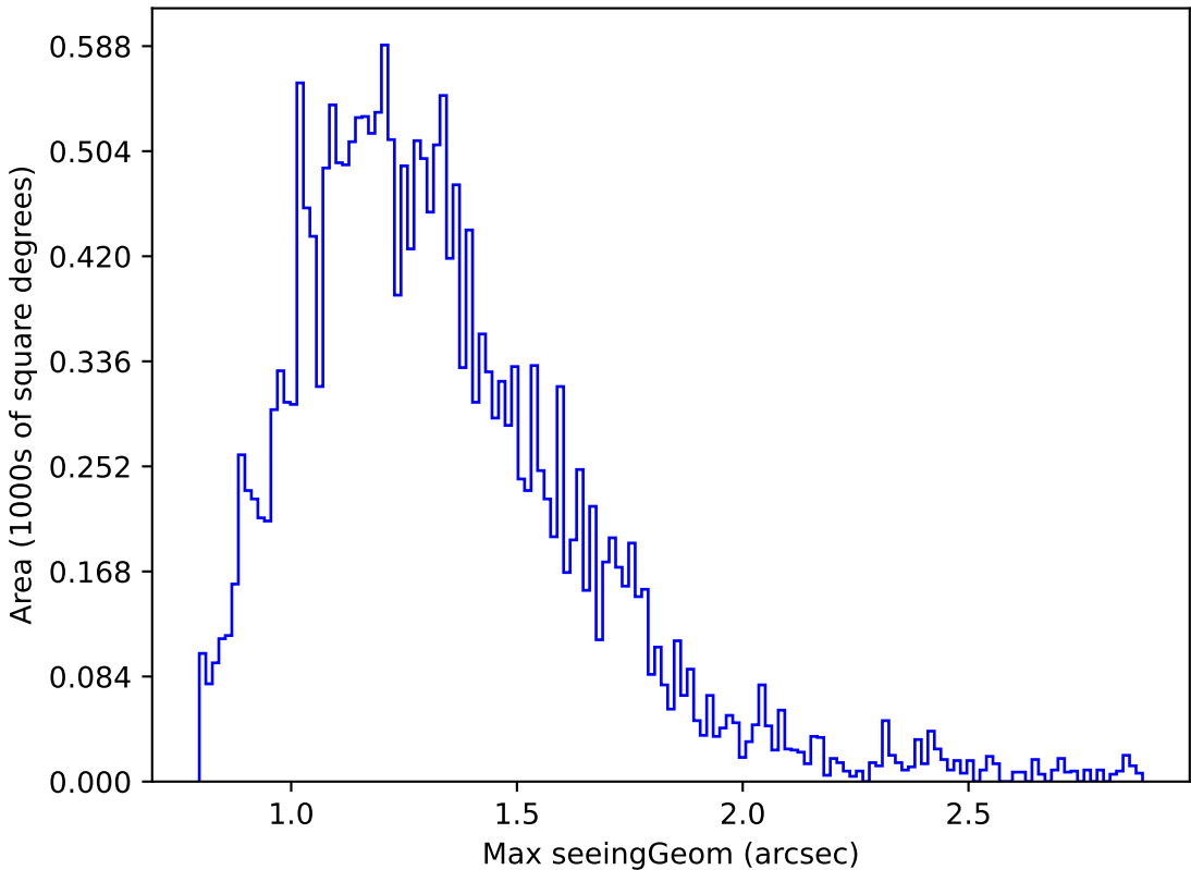
too_elab_r64_d3_gz_v3.4_10yrs Yr 1 u band: Max seeingGeom
