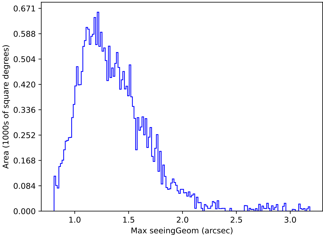
too_elab_r64_d3_gz_v3.4_10yrs Yr 1 g band: Max seeingGeom
