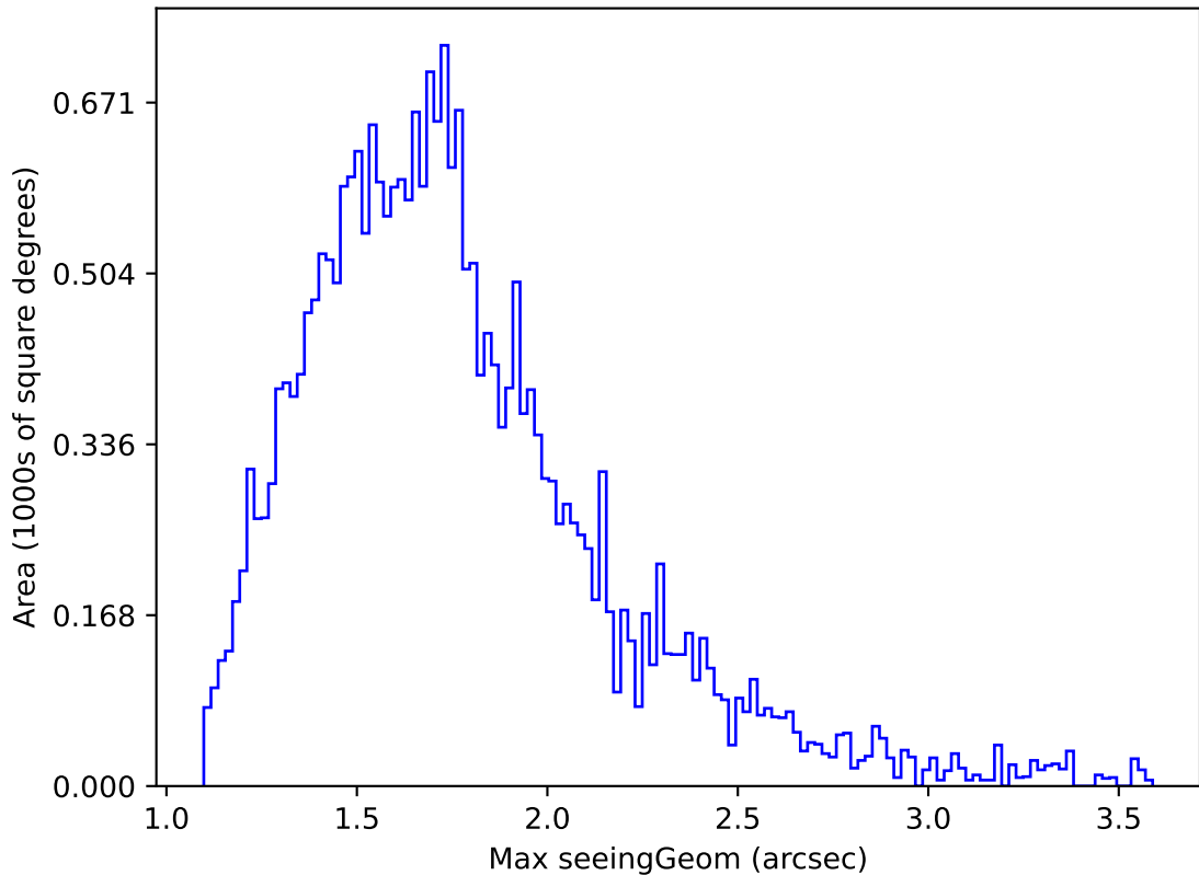
too_elab_r64_d3_gz_v3.4_10yrs Yr 1 all bands: Max seeingGeom
