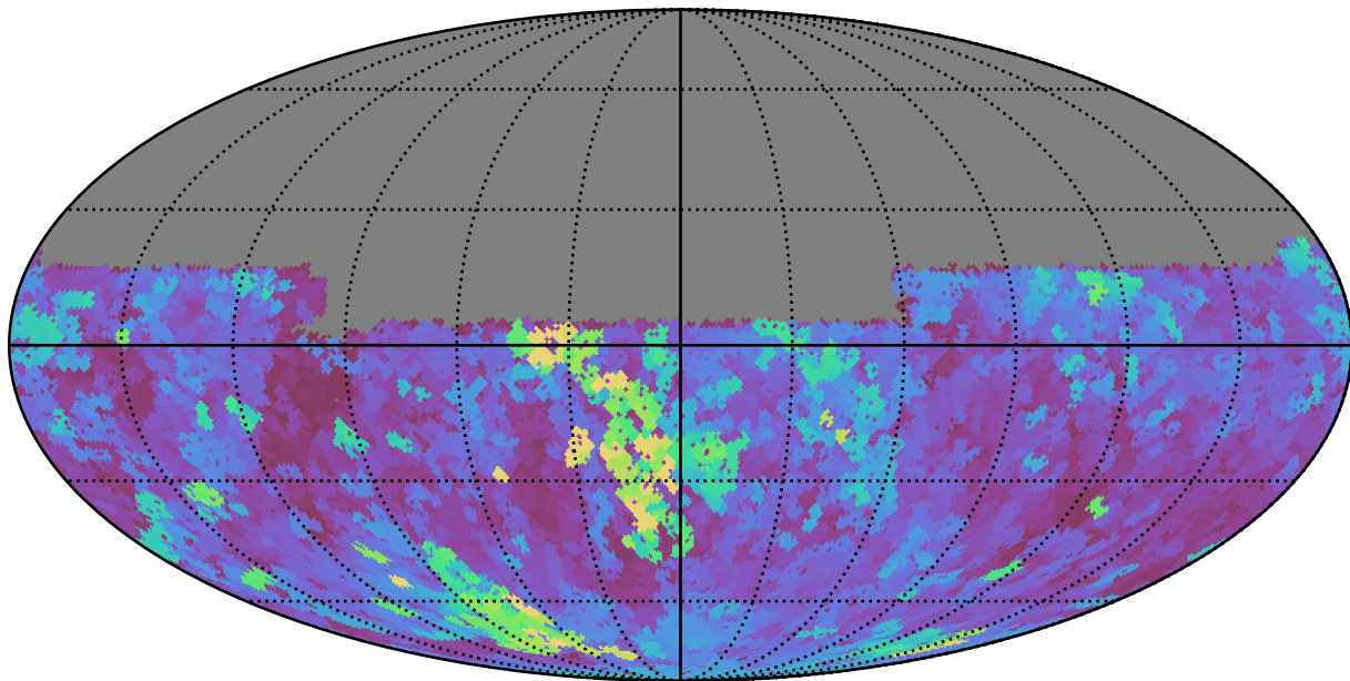
too_elab_r64_d3_gz_v3.4_10yrs Yr 1 y band: Max seeingEff
