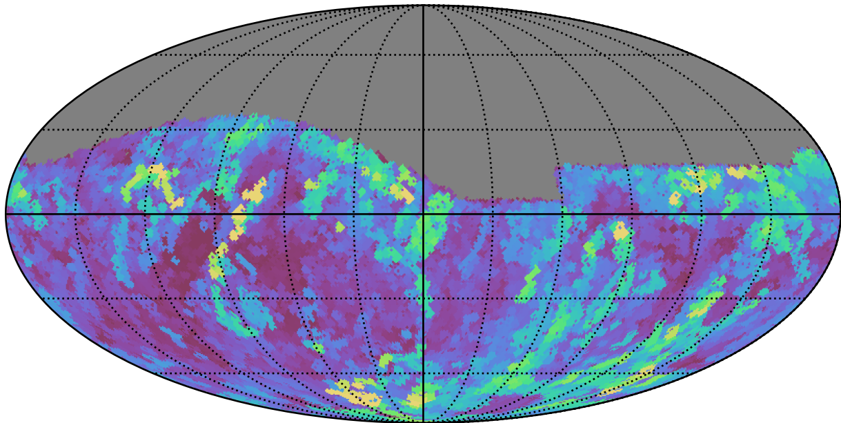
too_elab_r64_d3_gz_v3.4_10yrs Yr 1 r band: Max seeingEff
