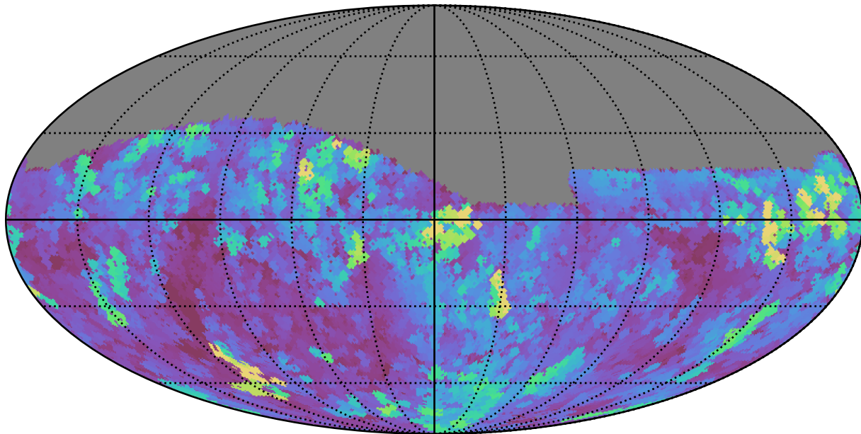
too_elab_r64_d3_gz_v3.4_10yrs Yr 1 i band: Max seeingEff
