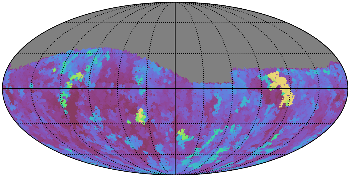
too_elab_r64_d3_gz_v3.4_10yrs Yr 1 g band: Max seeingEff
