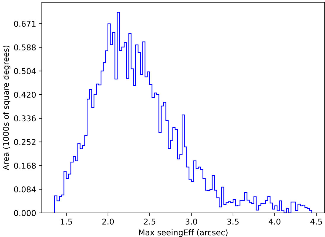
too_elab_r64_d3_gz_v3.4_10yrs All sky y band: Max seeingEff
