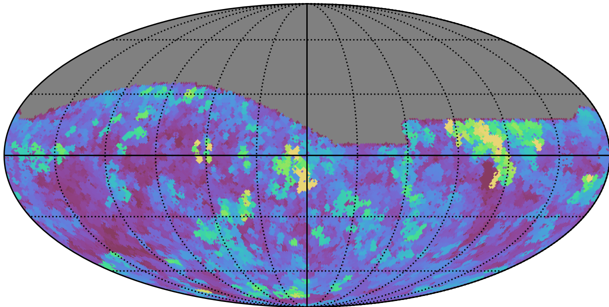
too_elab_r64_d3_gz_v3.4_10yrs All sky g band: Max seeingEff
