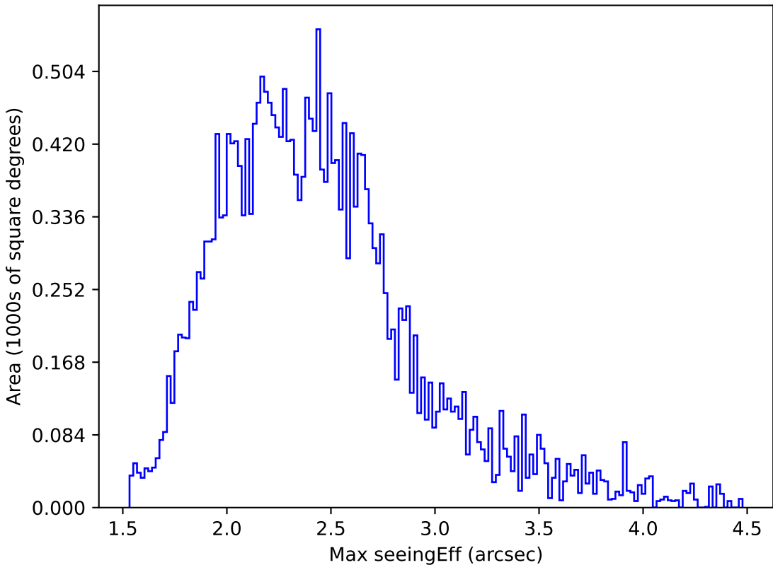
too_elab_r64_d3_gz_v3.4_10yrs All sky g band: Max seeingEff
