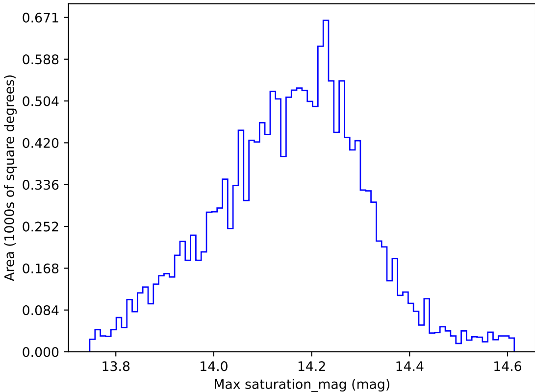
too_elab_r64_d3_gz_v3.4_10yrs WFD y band: Max saturation_mag
