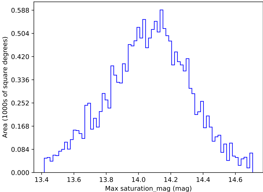
too_elab_r64_d3_gz_v3.4_10yrs WFD u band: Max saturation_mag
