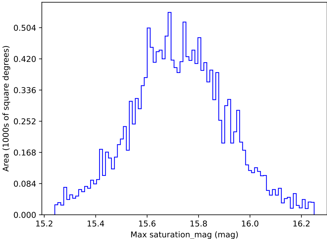
too_elab_r64_d3_gz_v3.4_10yrs WFD g band: Max saturation_mag
