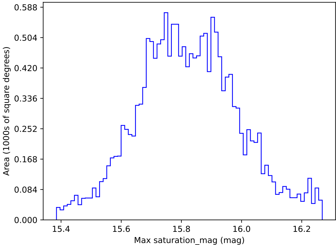
too_elab_r64_d3_gz_v3.4_10yrs WFD all bands: Max saturation_mag
