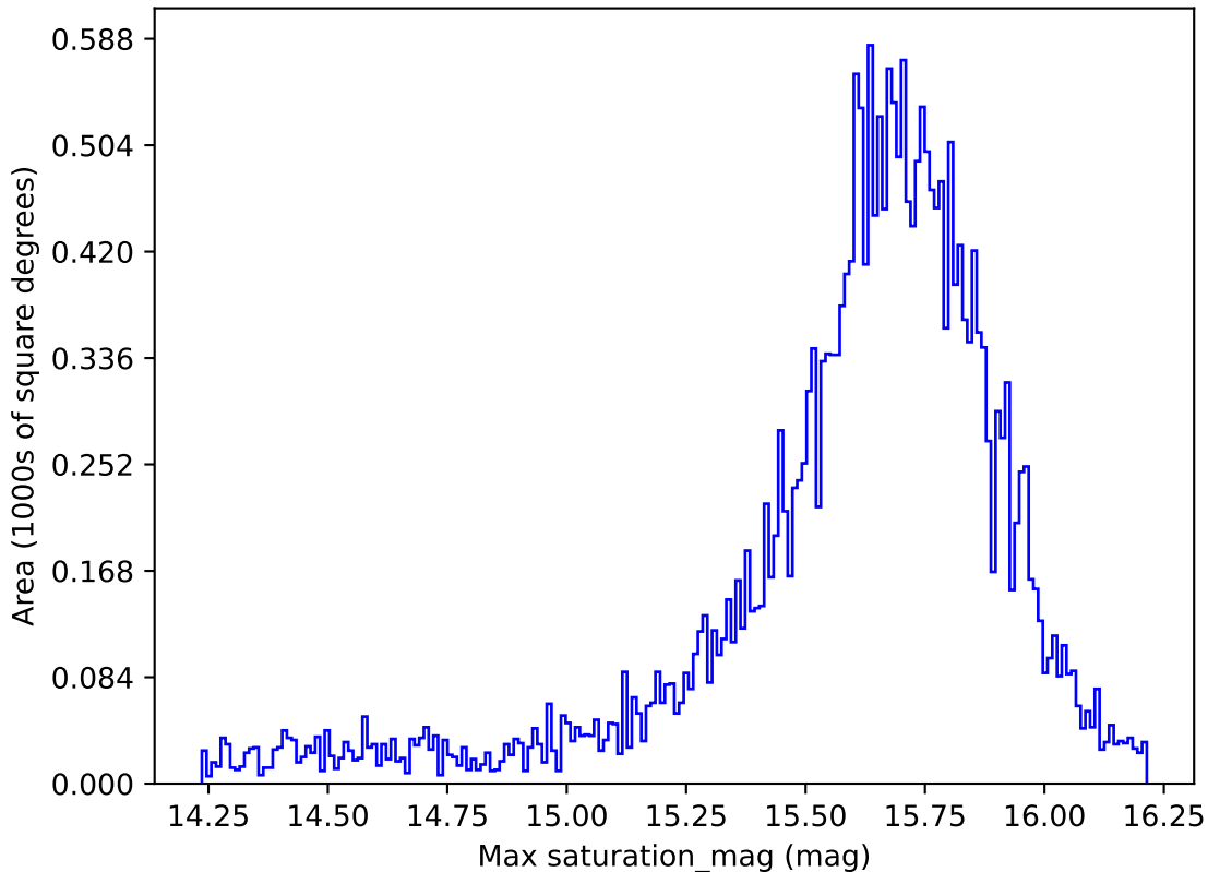
too_elab_r64_d3_gz_v3.4_10yrs All sky g band: Max saturation_mag
