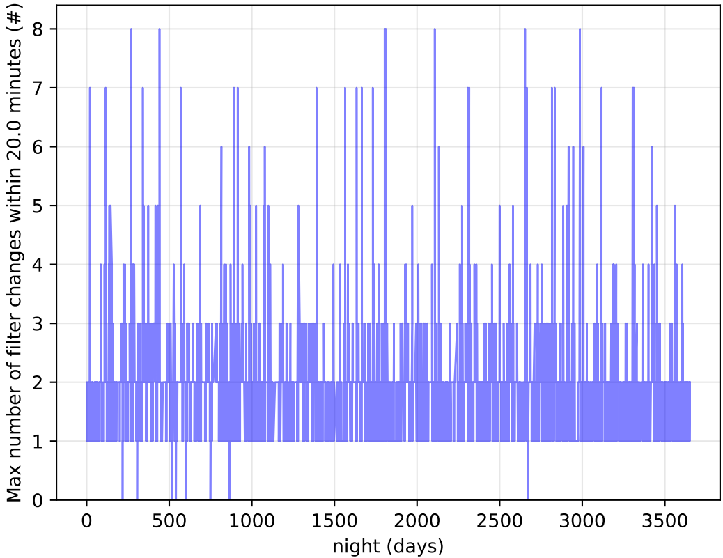
too_elab_r64_d3_gz_v3.4_10yrs Per Night: Max number of filter changes within 20.0 minutes
