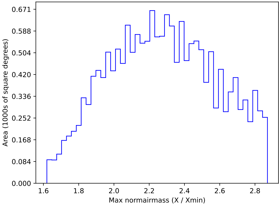
too_elab_r64_d3_gz_v3.4_10yrs WFD z band: Max normairmass
