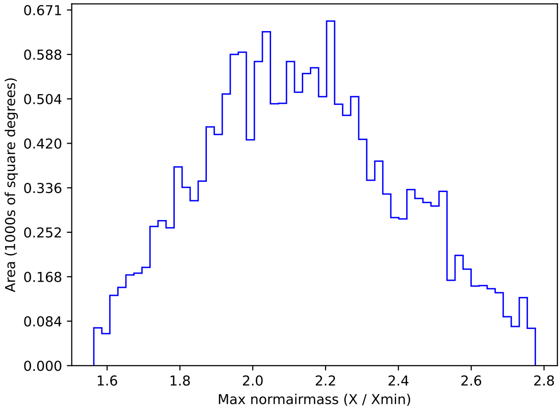
too_elab_r64_d3_gz_v3.4_10yrs WFD y band: Max normairmass
