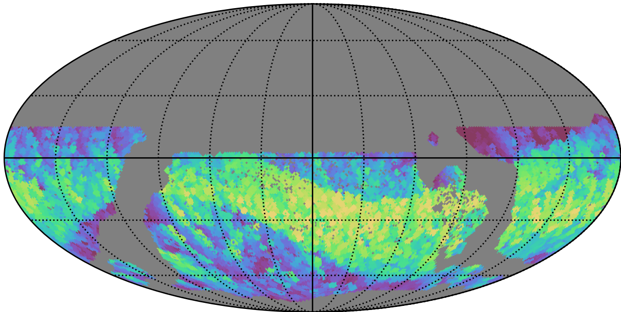
too_elab_r64_d3_gz_v3.4_10yrs WFD i band: Max normairmass
