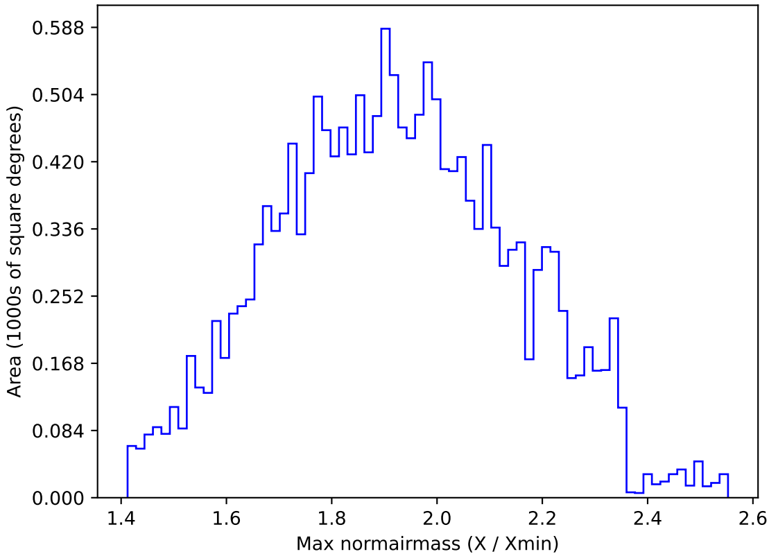
too_elab_r64_d3_gz_v3.4_10yrs WFD g band: Max normairmass
