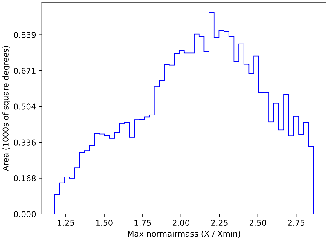
too_elab_r64_d3_gz_v3.4_10yrs All sky z band: Max normairmass
