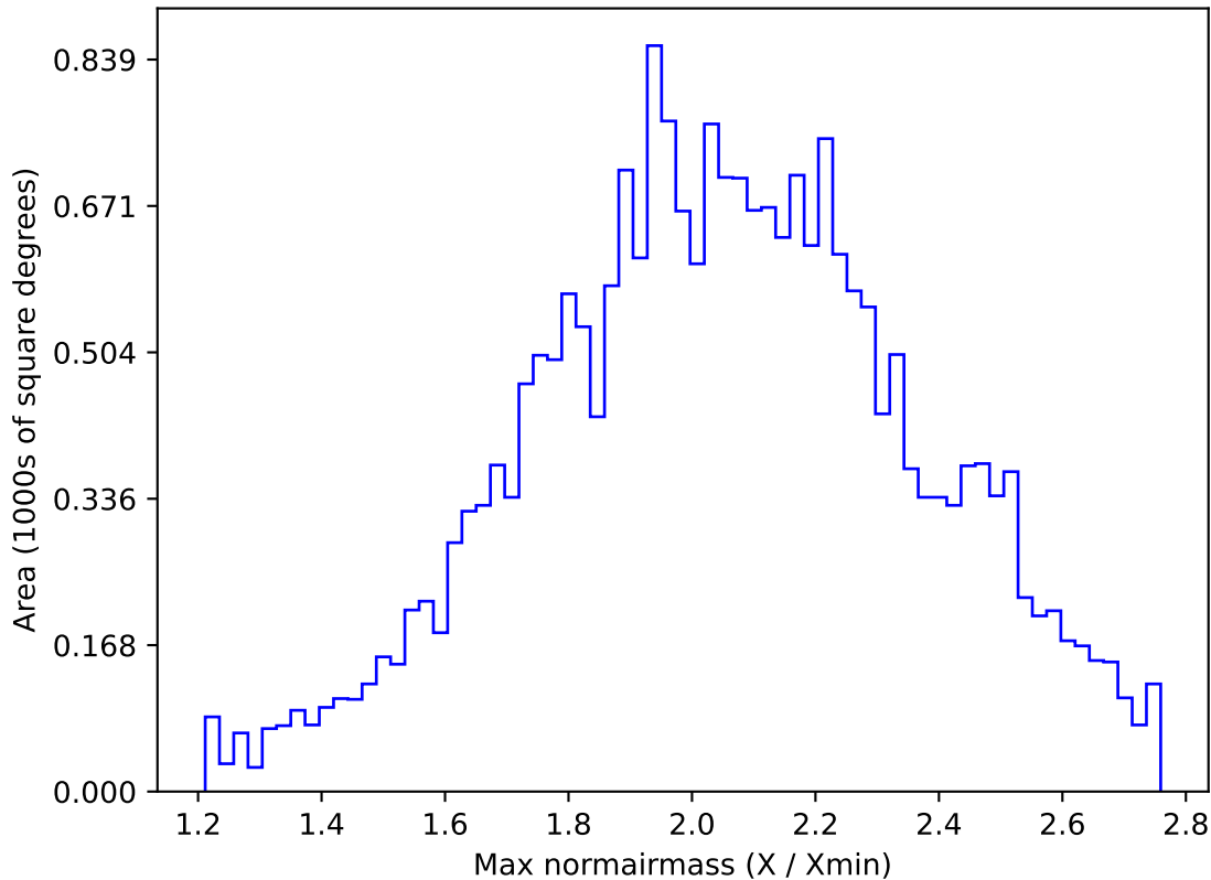
too_elab_r64_d3_gz_v3.4_10yrs All sky y band: Max normairmass
