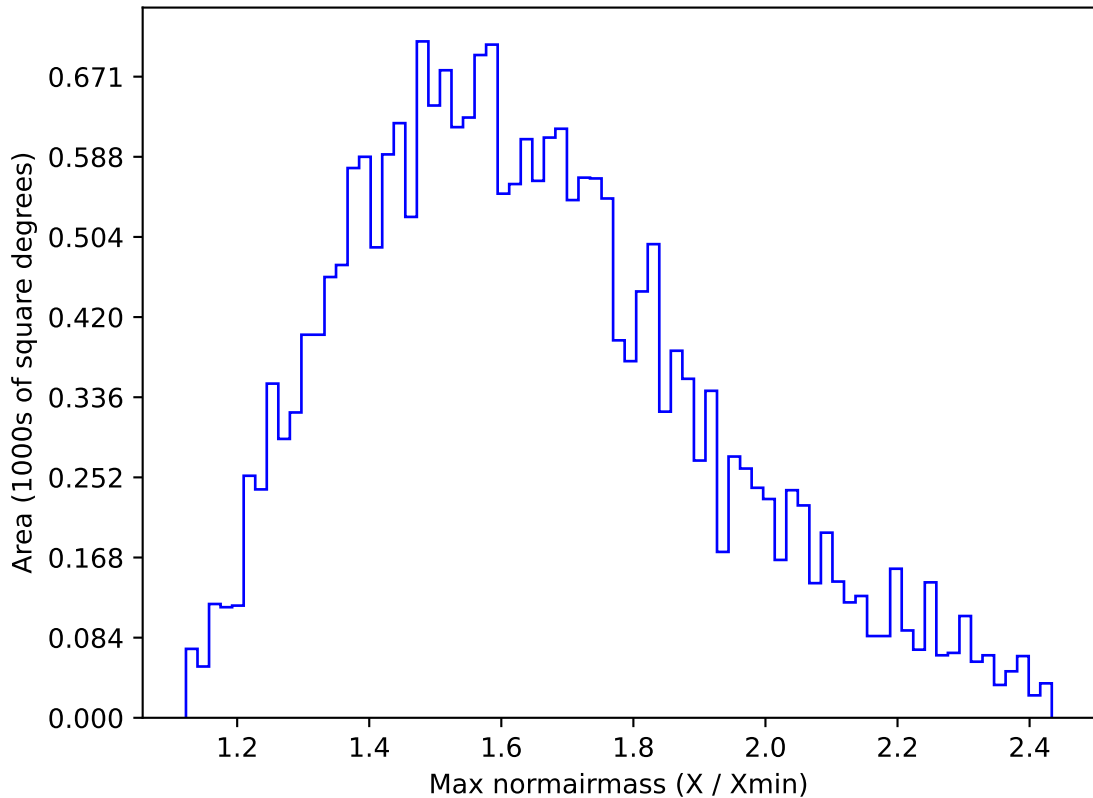
too_elab_r64_d3_gz_v3.4_10yrs All sky u band: Max normairmass
