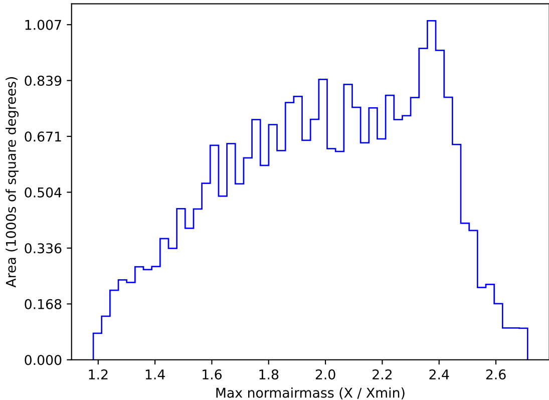
too_elab_r64_d3_gz_v3.4_10yrs All sky r band: Max normairmass
