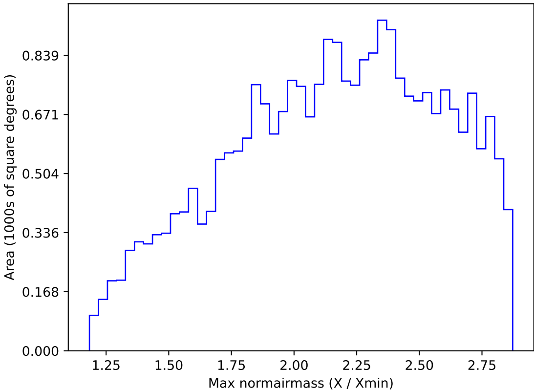
too_elab_r64_d3_gz_v3.4_10yrs All sky i band: Max normairmass
