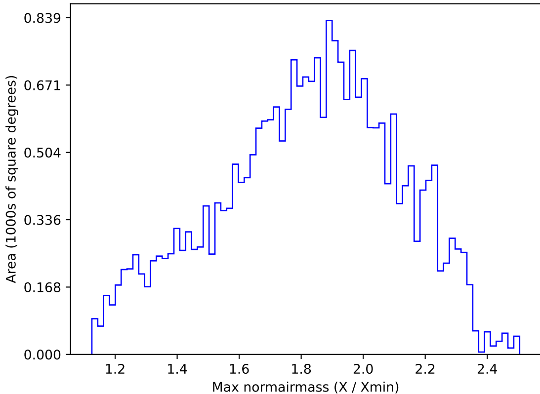
too_elab_r64_d3_gz_v3.4_10yrs All sky g band: Max normairmass
