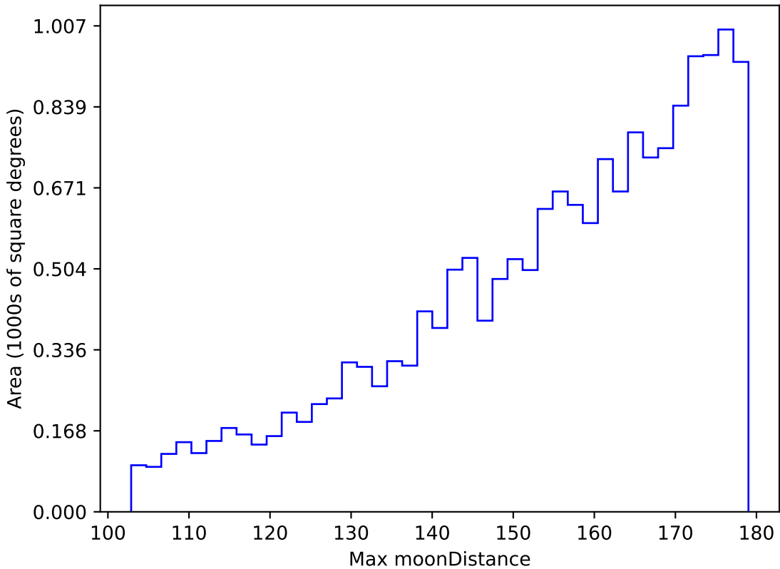
too_elab_r64_d3_gz_v3.4_10yrs WFD z band: Max moonDistance
