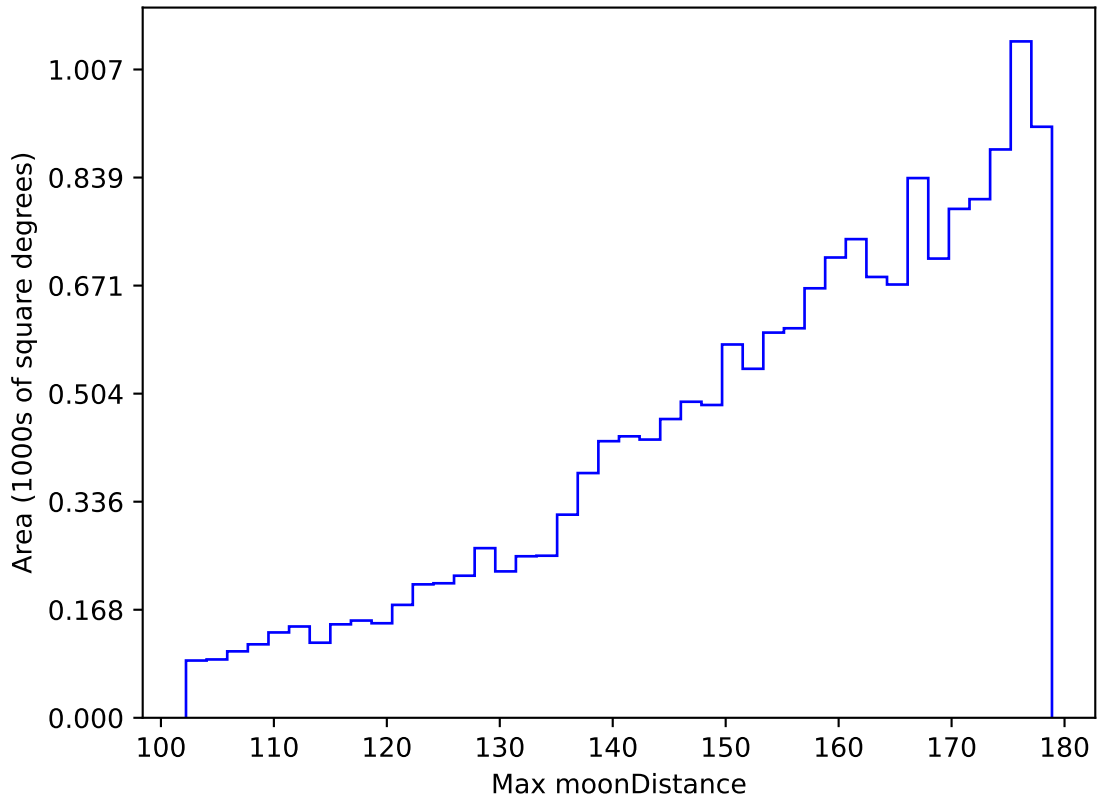
too_elab_r64_d3_gz_v3.4_10yrs WFD u band: Max moonDistance
