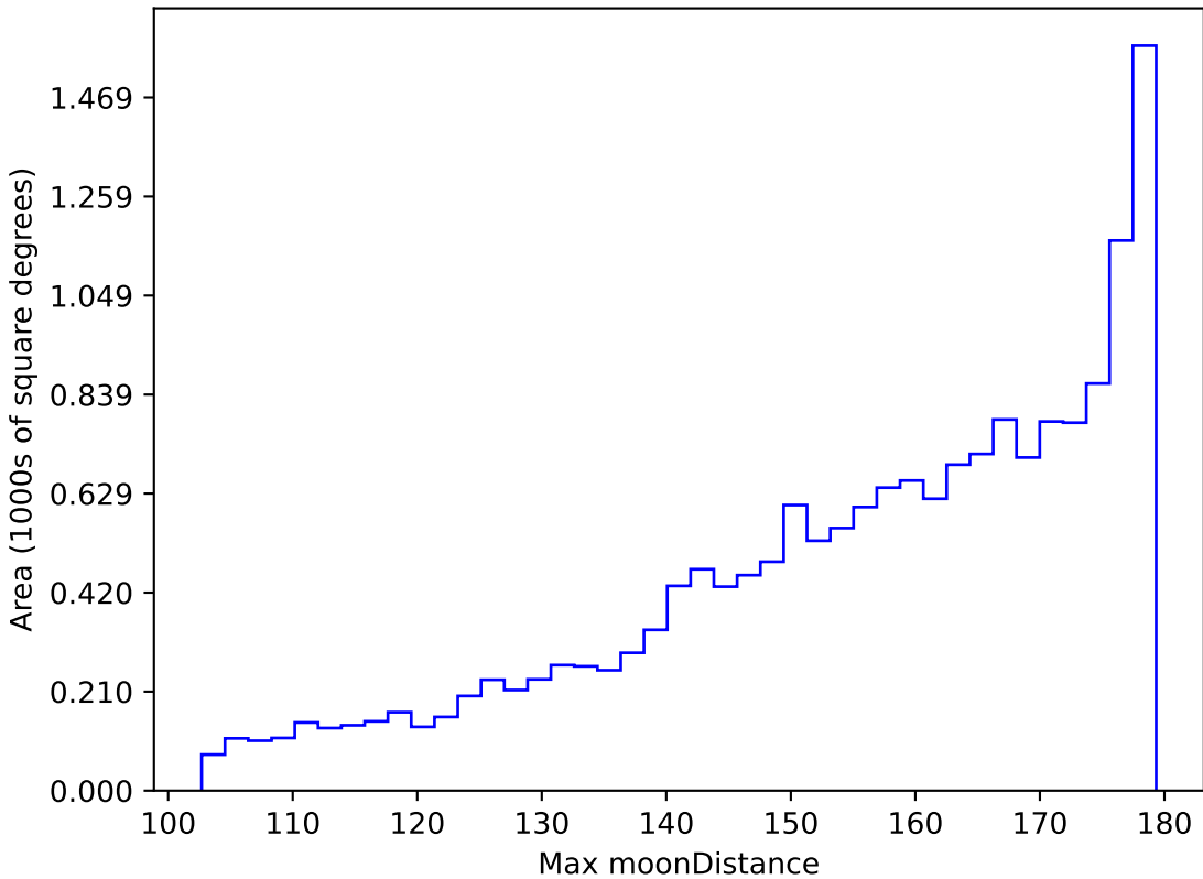
too_elab_r64_d3_gz_v3.4_10yrs WFD r band: Max moonDistance
