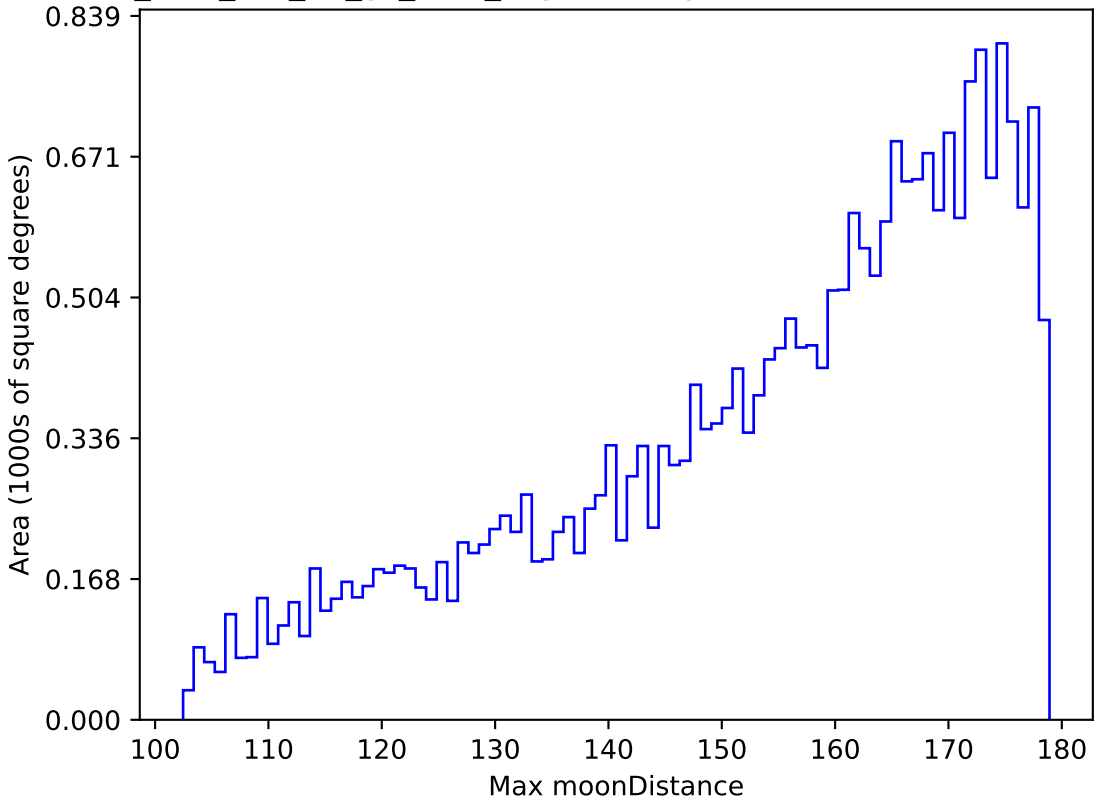
too_elab_r64_d3_gz_v3.4_10yrs All sky z band: Max moonDistance
