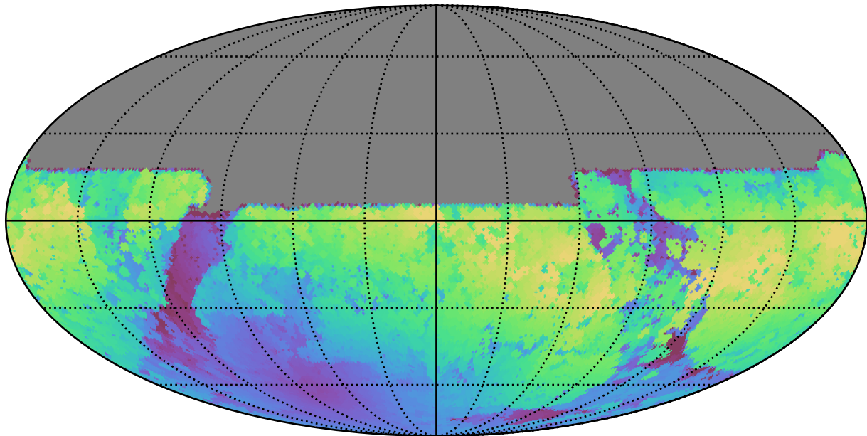
too_elab_r64_d3_gz_v3.4_10yrs All sky y band: Max moonDistance
