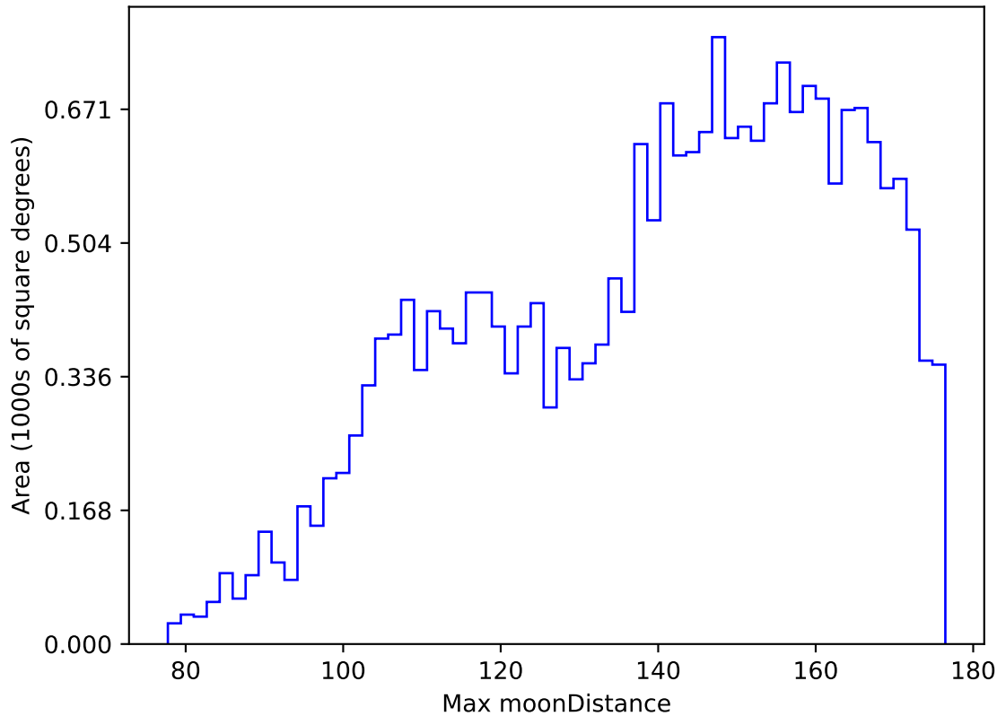
too_elab_r64_d3_gz_v3.4_10yrs All sky y band: Max moonDistance
