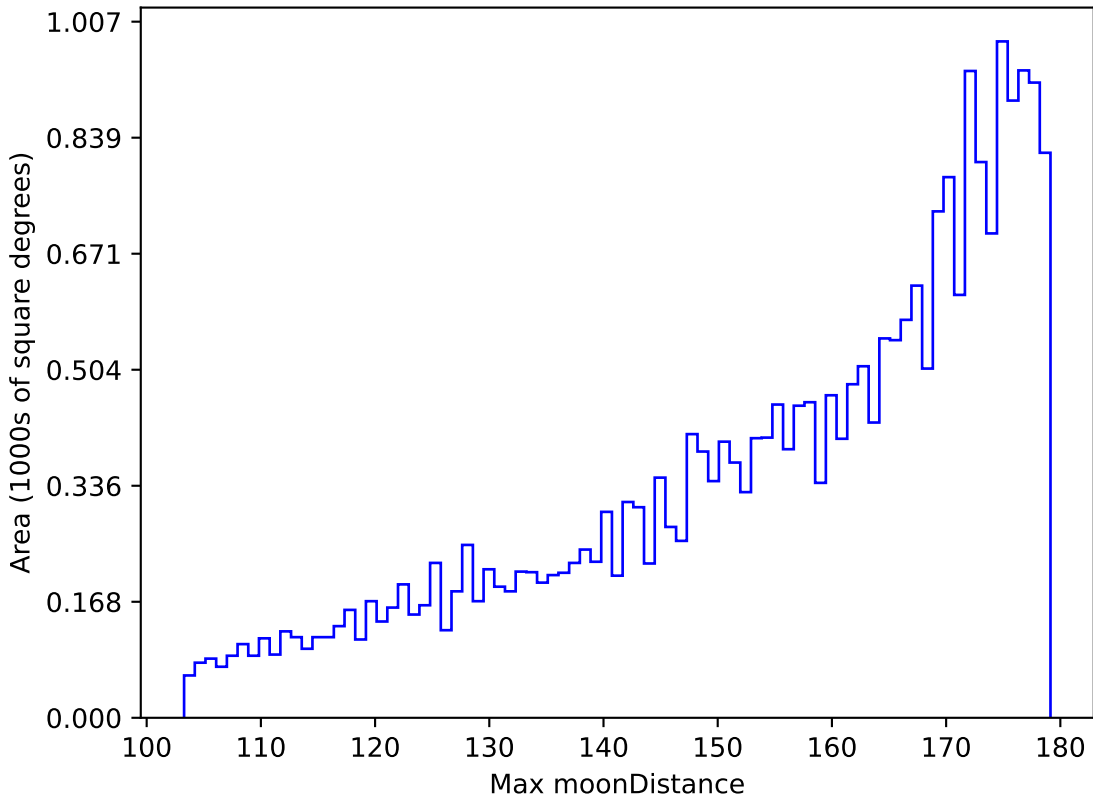
too_elab_r64_d3_gz_v3.4_10yrs All sky i band: Max moonDistance
