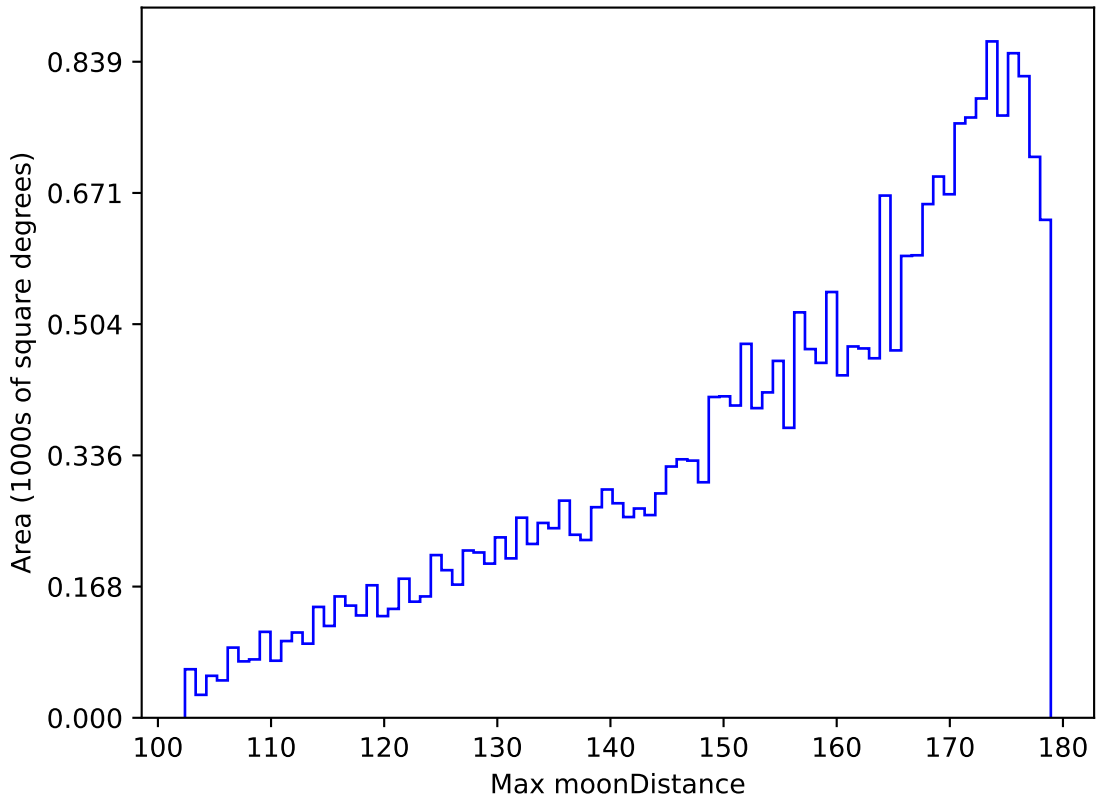
too_elab_r64_d3_gz_v3.4_10yrs All sky g band: Max moonDistance
