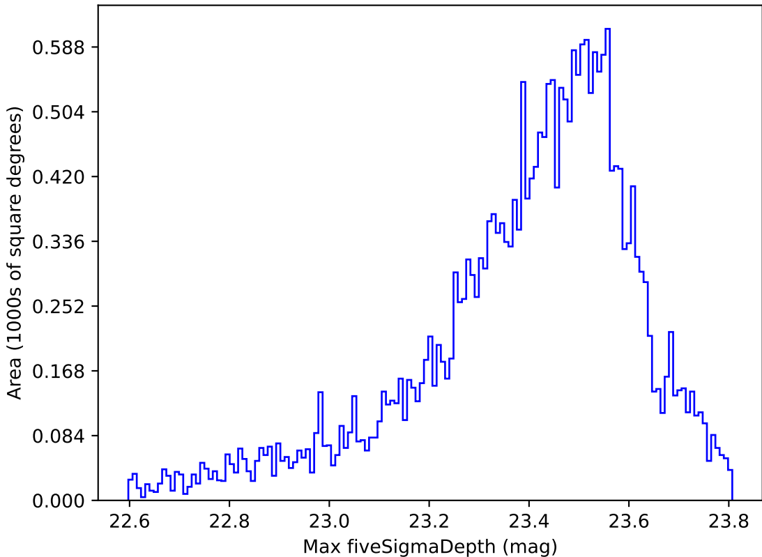
too_elab_r64_d3_gz_v3.4_10yrs Yr 1 z band: Max fiveSigmaDepth
