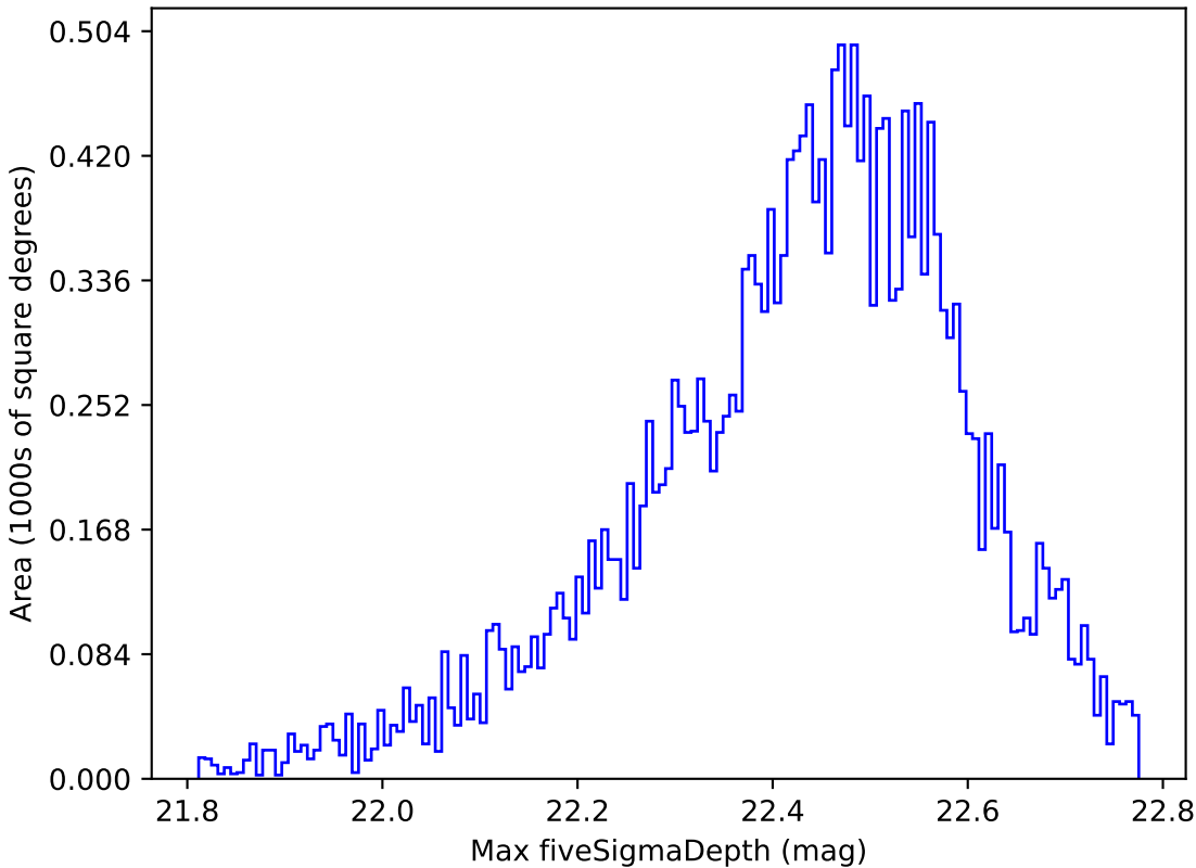
too_elab_r64_d3_gz_v3.4_10yrs Yr 1 y band: Max fiveSigmaDepth
