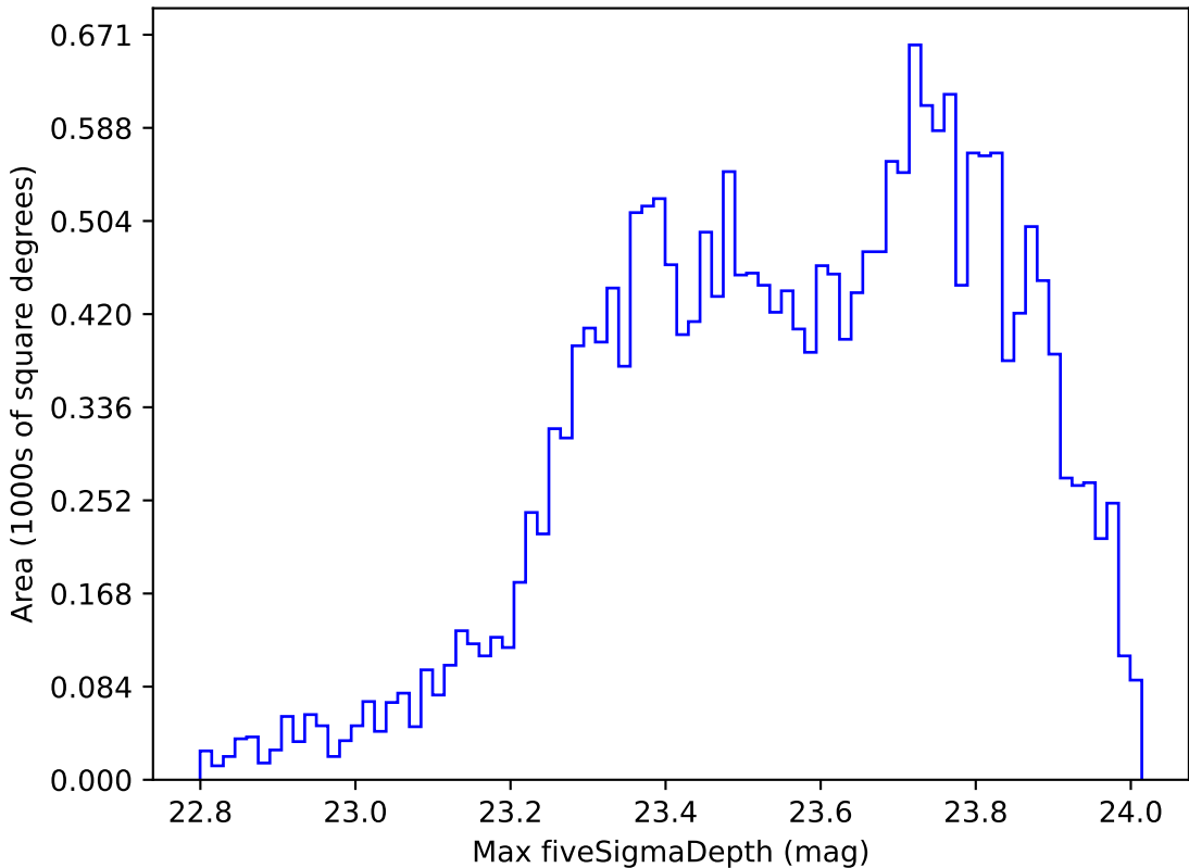
too_elab_r64_d3_gz_v3.4_10yrs Yr 1 u band: Max fiveSigmaDepth
