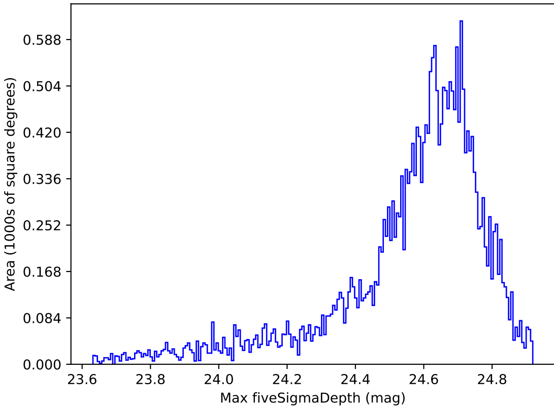
too_elab_r64_d3_gz_v3.4_10yrs Yr 1 r band: Max fiveSigmaDepth
